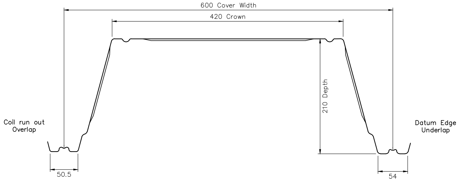
SECTION THROUGH PROFILE
