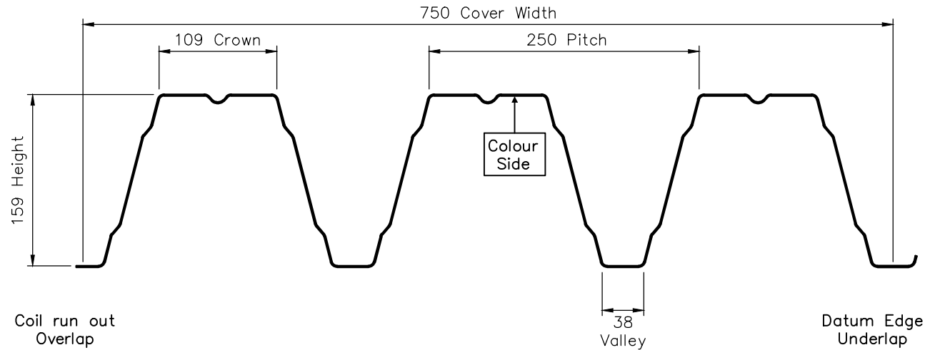
SECTION THROUGH PROFILE
