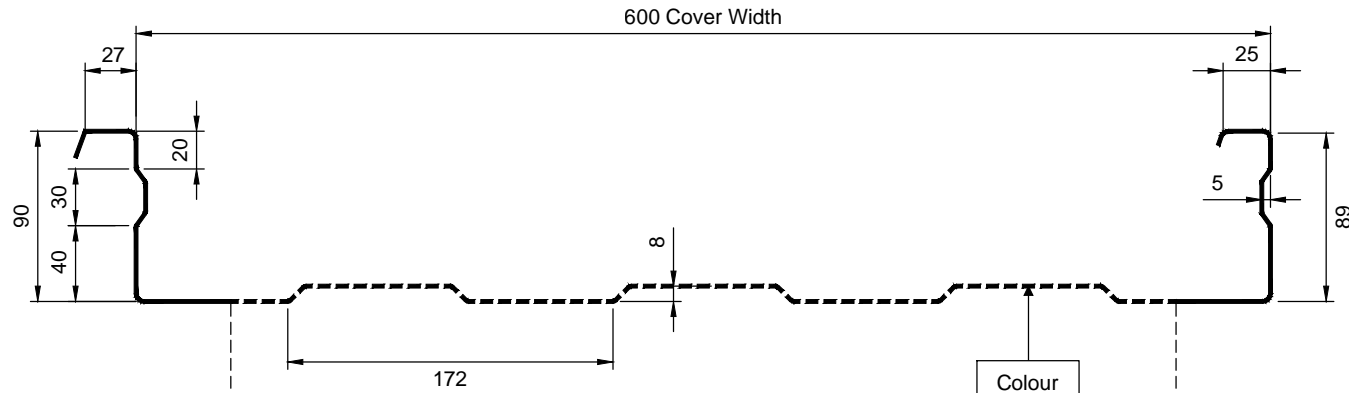
SECTION THROUGH PROFILE
