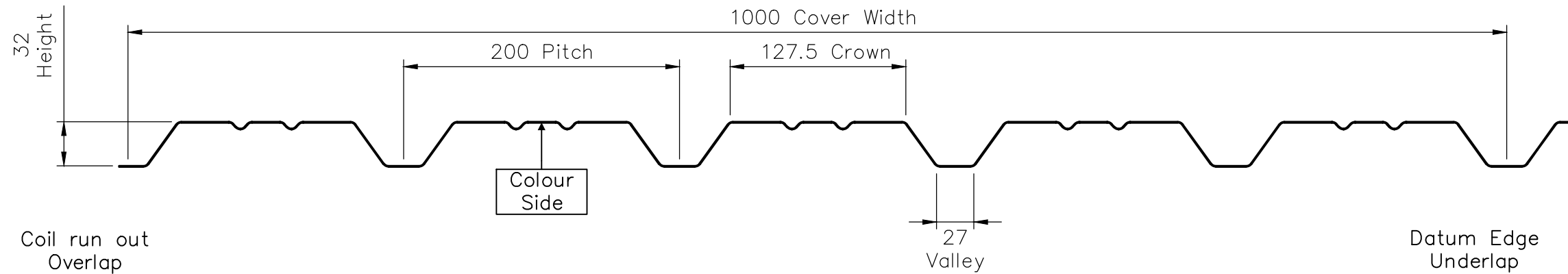
SECTION THROUGH PROFILE
