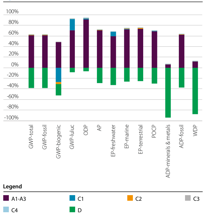
Figure 4 LCA results for steel structural hollow sections
